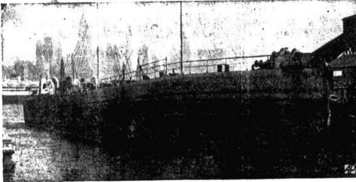
WHAT IT DOESN'T HAVE makes this all-welded motor ship, Dolomite, seen in N. Y., unusual. The ship is keel-less, ribless and rivetless and has five cargo holds lined with nickel.
